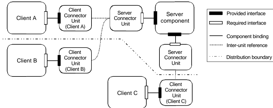
Fig. 6. Application architecture after transformation of the enhanced description
