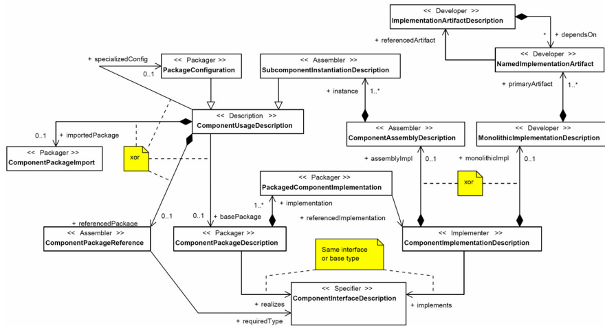
Fig. 3. An overview of the component data model
